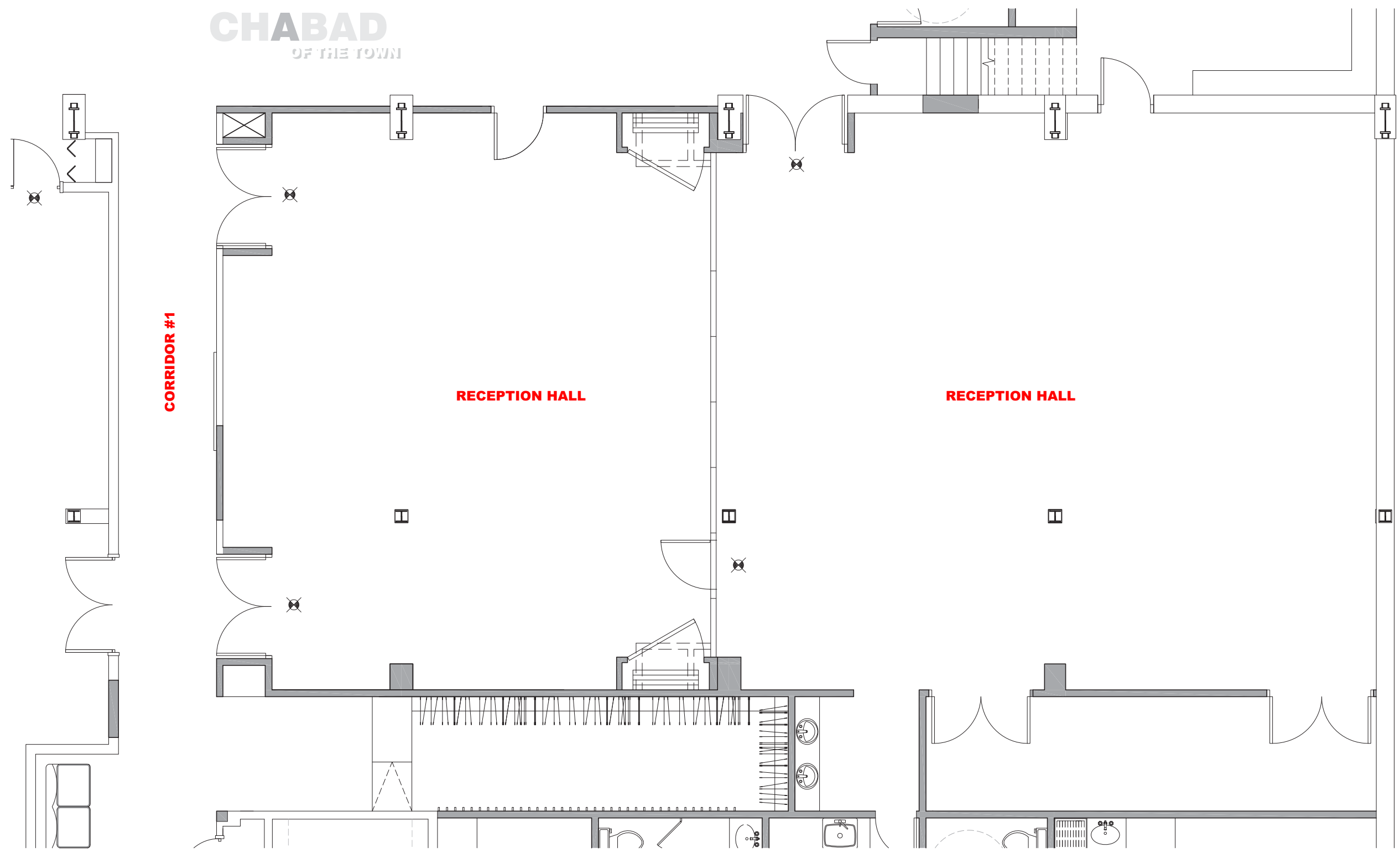
RECEPTION HALL LAYOUT
