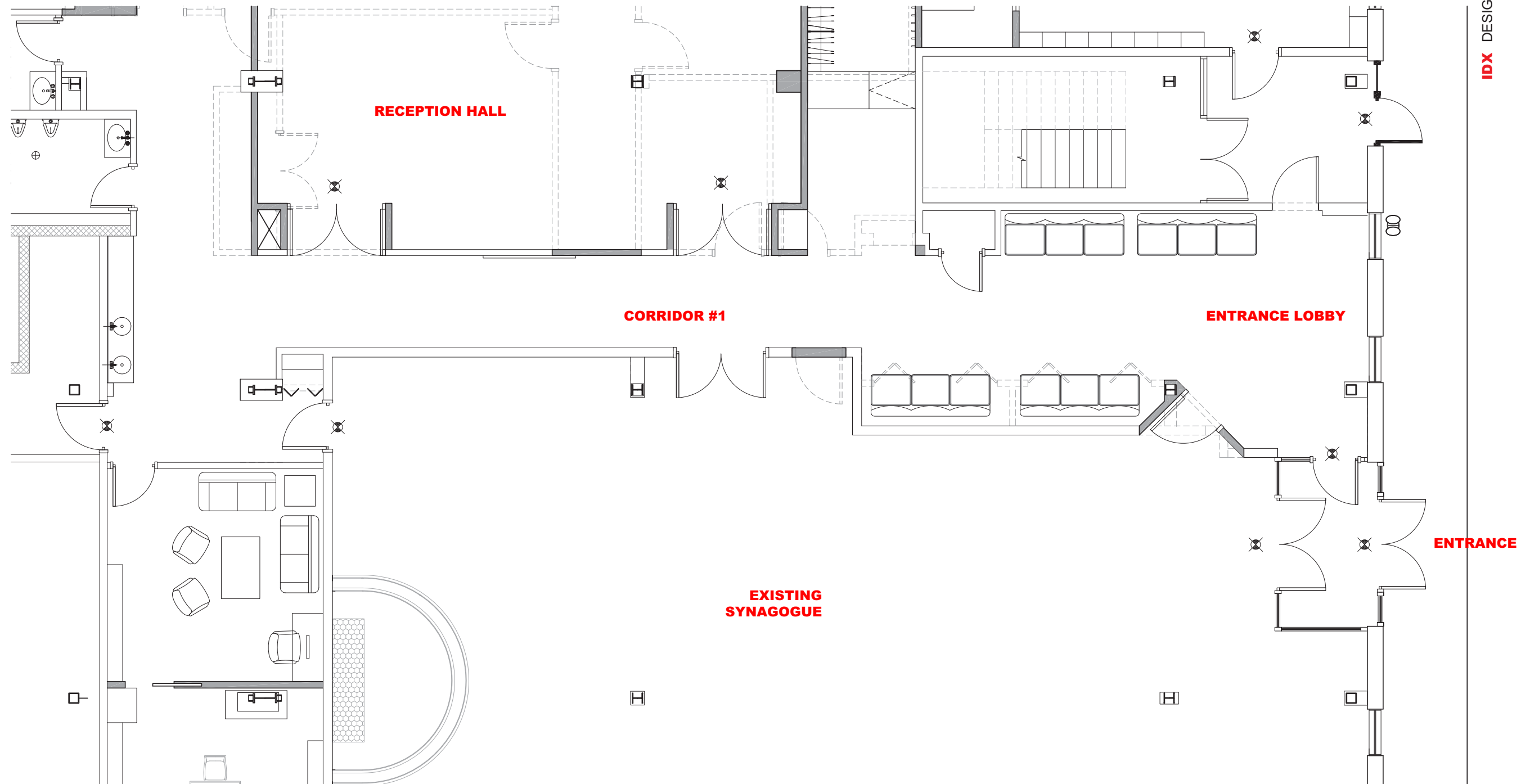
BUILDING LAYOUT
